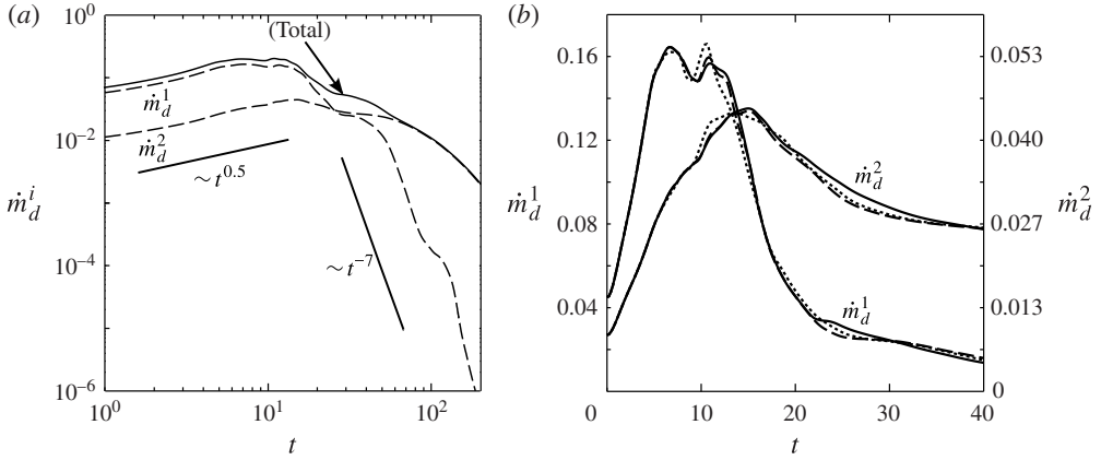
FIGURE 5. Time history of particle sedimentation rate for coarse ( \dot{m}_d^1 ) and fine ( \dot{m}_d^2 ) particles. (a) Case B1 shown on a logarithmic scale. (b) Comparison of all cases, where dotted, dashed and solid lines represent cases FL, B1 and B2, respectively.
