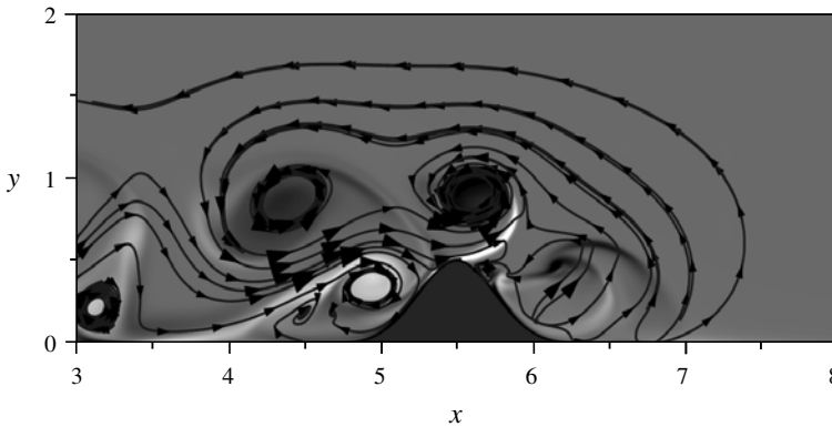
FIGURE 15. In-plane streamlines plotted in the symmetry plane z = 1.5 , at t = 11 for case B2. Background shading represents the out-of-plane vorticity component w_z (black corresponding to +15 , white to -15 and grey to zero). The separation and reattachment of the front are visible.
