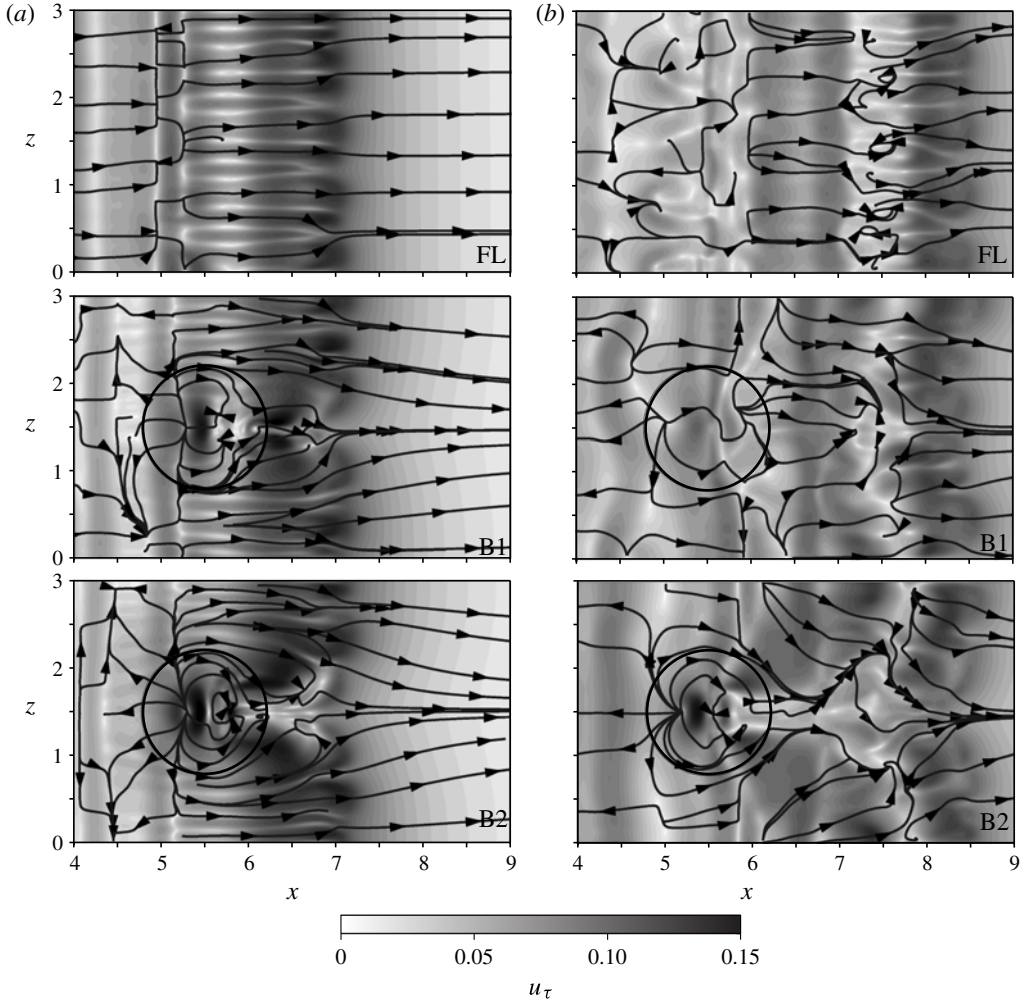
FIGURE 22. Magnitude of the friction velocity u_\tau (grey shading) for cases FL, B1 and B2 at times (a) t = 10.8 and (b) t = 14 . The lines represent the directional field of the instantaneous wall-shear stress. The vortical structures in the wake of the bump strongly modify the friction velocity field.
