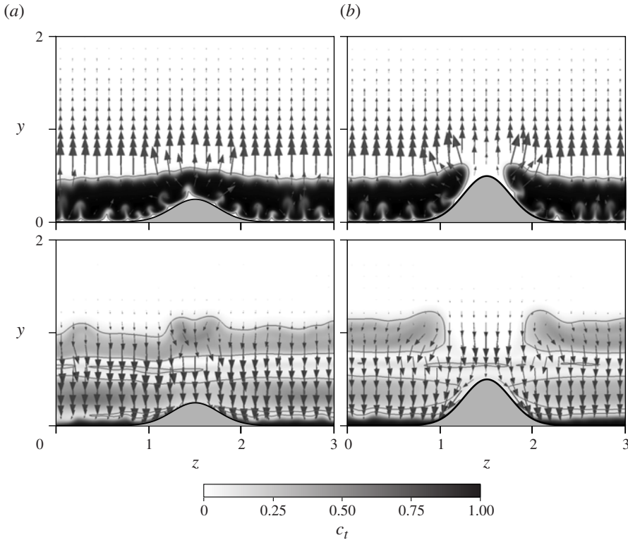
FIGURE 10. Evolution of currents (a) B1 and (b) B2 in the plane of the peak of the bump at x=5.5 . The top row corresponds to t=8 , whereas the bottom row depicts the currents for t=12 . The in-plane v, w -velocity vectors are also shown. The grey shading represents the total concentration field c_t , with the line showing the contour c_t=0.1 . While B1 passes over the bump, B2 mostly flows around the bump.
