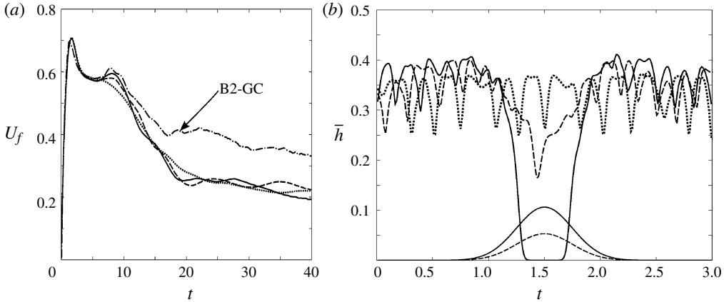
FIGURE 27. (a) Time history of the front velocities for currents FL (dots), B1 (dashed line), B2 (solid line) and B2-GC (dash-dotted line). As the current arrives at the bump and is deflected laterally, its height increases in the regions to the side of the bump, which in turn results in an increase of the front velocity. (b) Current height \bar{h} in the plane x = 5.5 shown at t = 8 . Dots, dashed line and solid lines represent cases FL, B1 and B2, respectively. The current height is reduced above the bump, but increases in the regions to the side of the bump. Consequently, the streamwise hydrostatic pressure gradient driving the flow increases in these regions, and the current front accelerates.
