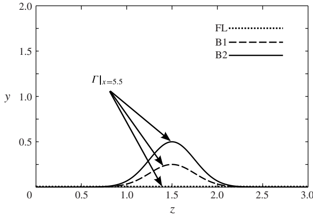
FIGURE 2. Cross-sections of the bottom topography ( \Gamma ) in simulations FL, B1 and B2, corresponding to a flat bottom, and bump heights equal to h = 0.25 and h = 0.5 , respectively. The y, z plane is shown at the streamwise location of the bumps peak, x = 5.5 .
